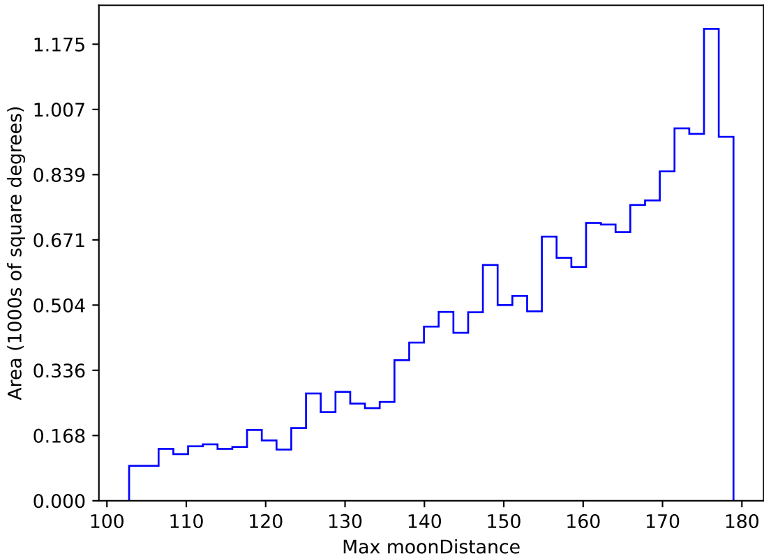
too_elab_r16_d2_ugrizy_v3.4_10yrs WFD g band: Max moonDistance
