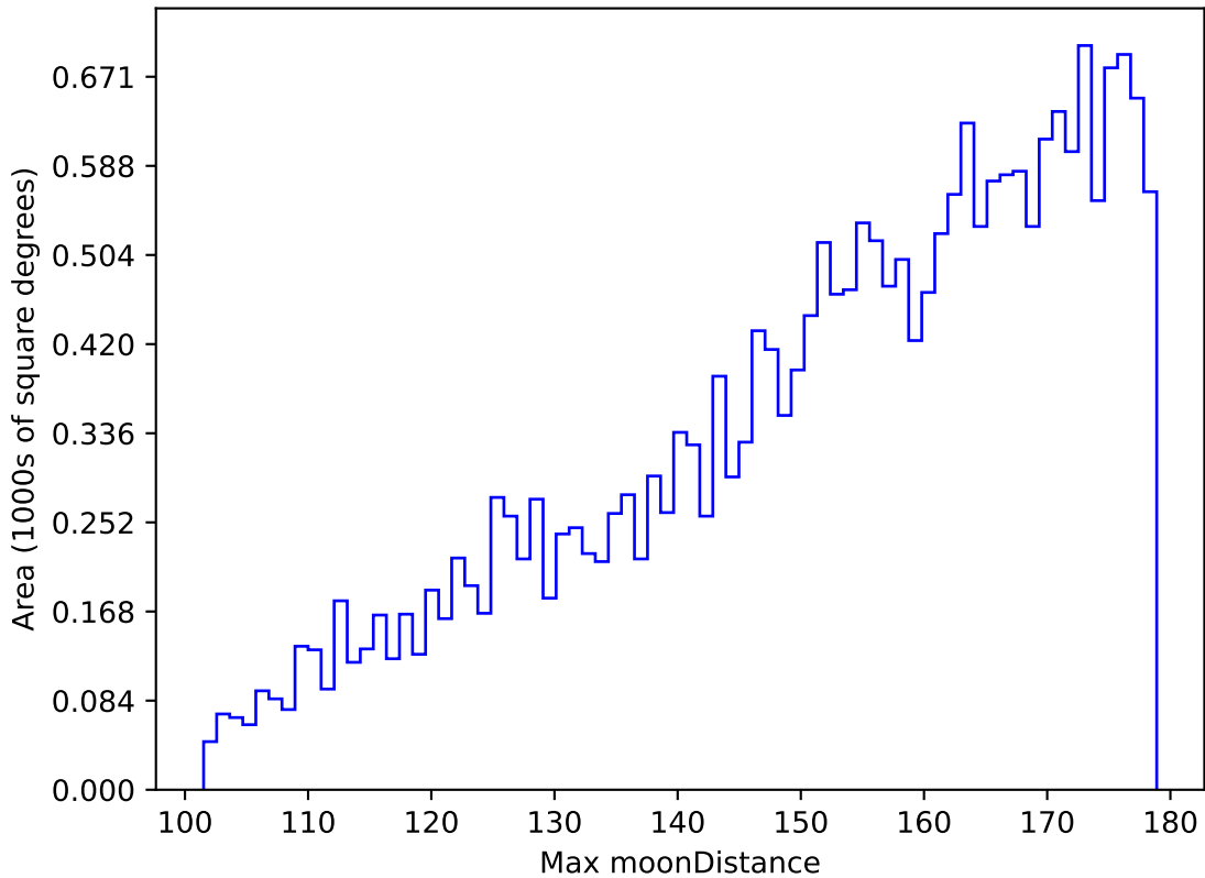
too_elab_r16_d2_ugrizy_v3.4_10yrs All sky u band: Max moonDistance
