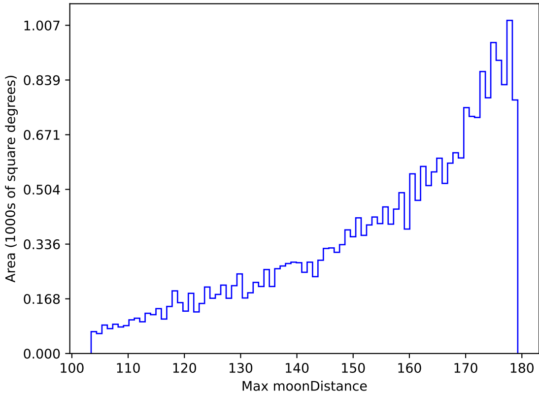
too_elab_r16_d2_ugrizy_v3.4_10yrs All sky i band: Max moonDistance
