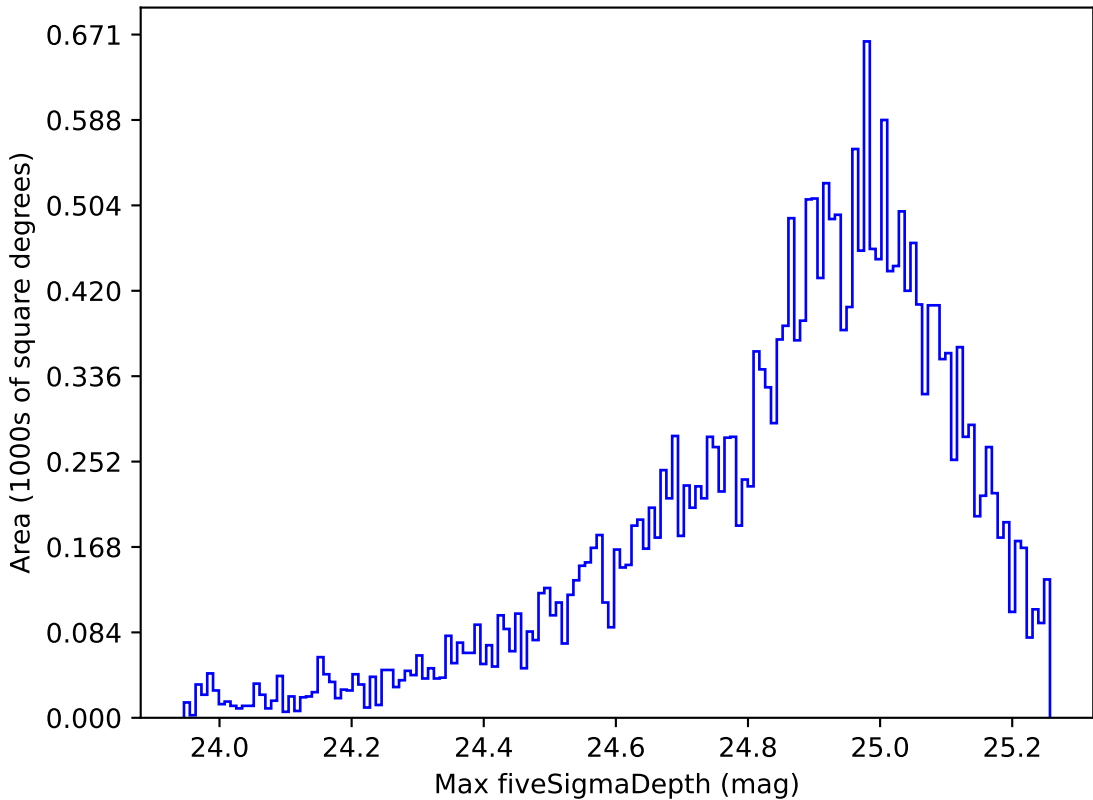
too_elab_r16_d2_ugrizy_v3.4_10yrs Yr 1 g band: Max fiveSigmaDepth
