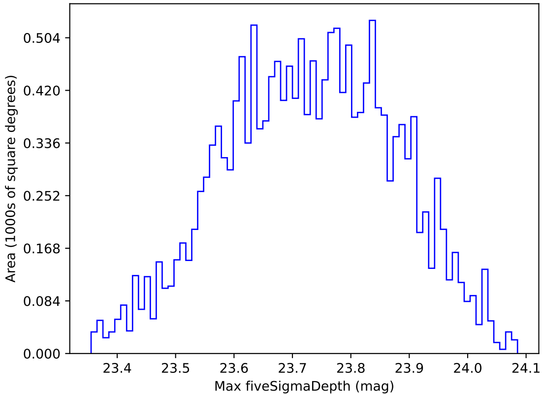
too_elab_r16_d2_ugrizy_v3.4_10yrs WFD u band: Max fiveSigmaDepth
