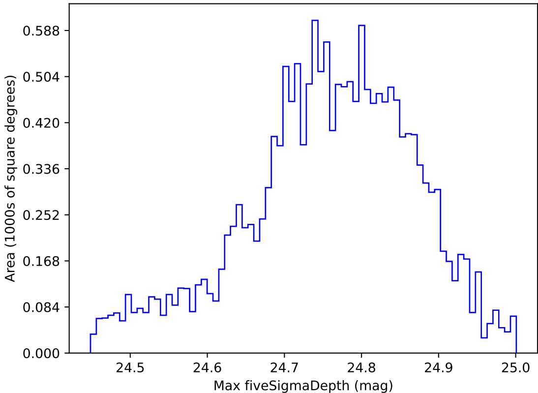
too_elab_r16_d2_ugrizy_v3.4_10yrs WFD r band: Max fiveSigmaDepth
