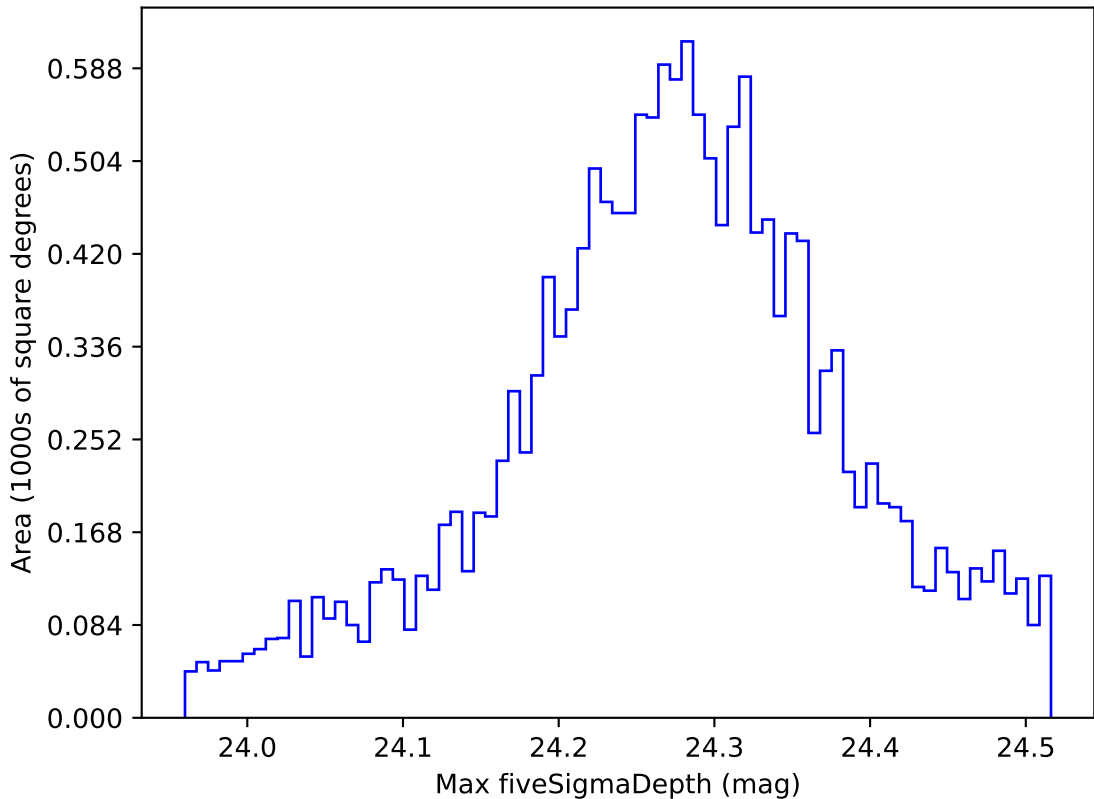
too_elab_r16_d2_ugrizy_v3.4_10yrs WFD i band: Max fiveSigmaDepth
