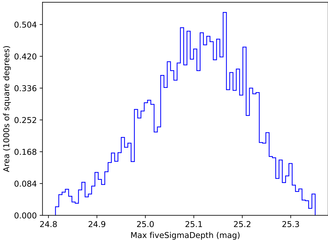
too_elab_r16_d2_ugrizy_v3.4_10yrs WFD g band: Max fiveSigmaDepth
