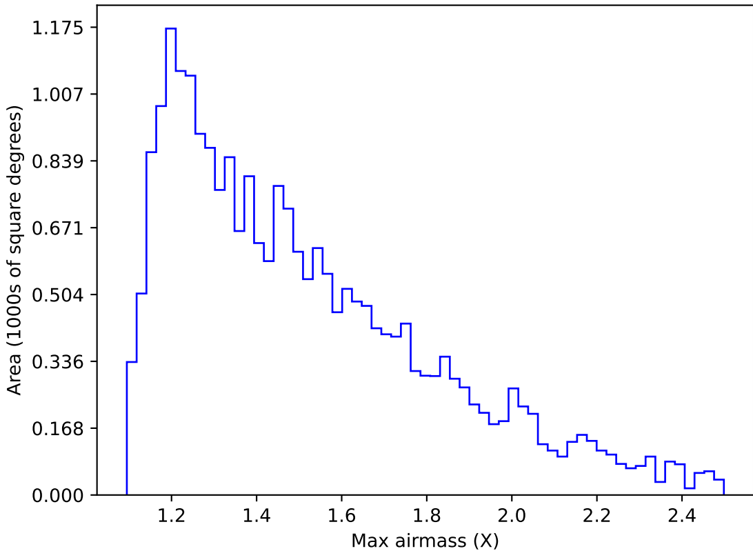
too_elab_r16_d2_ugrizy_v3.4_10yrs Yr 1 u band: Max airmass
