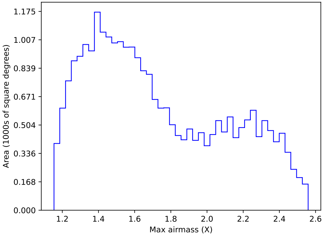
too_elab_r16_d2_ugrizy_v3.4_10yrs Yr 1 r band: Max airmass
