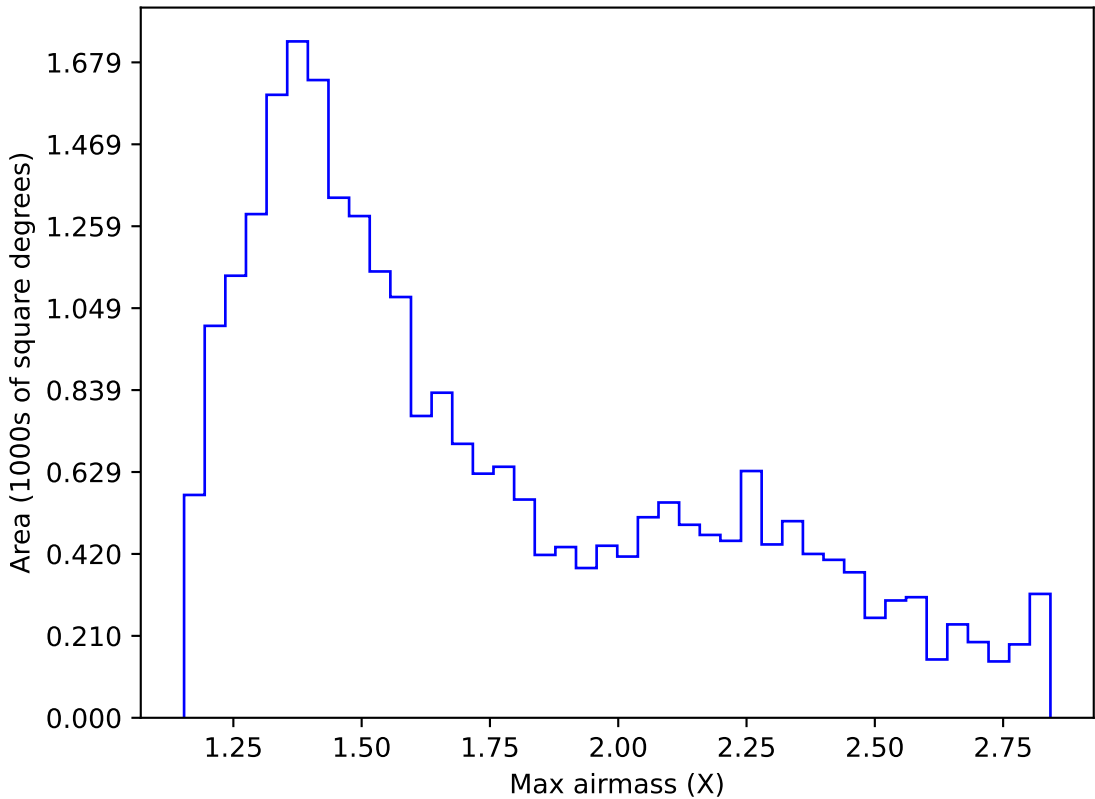
too_elab_r16_d2_ugrizy_v3.4_10yrs Yr 1 i band: Max airmass
