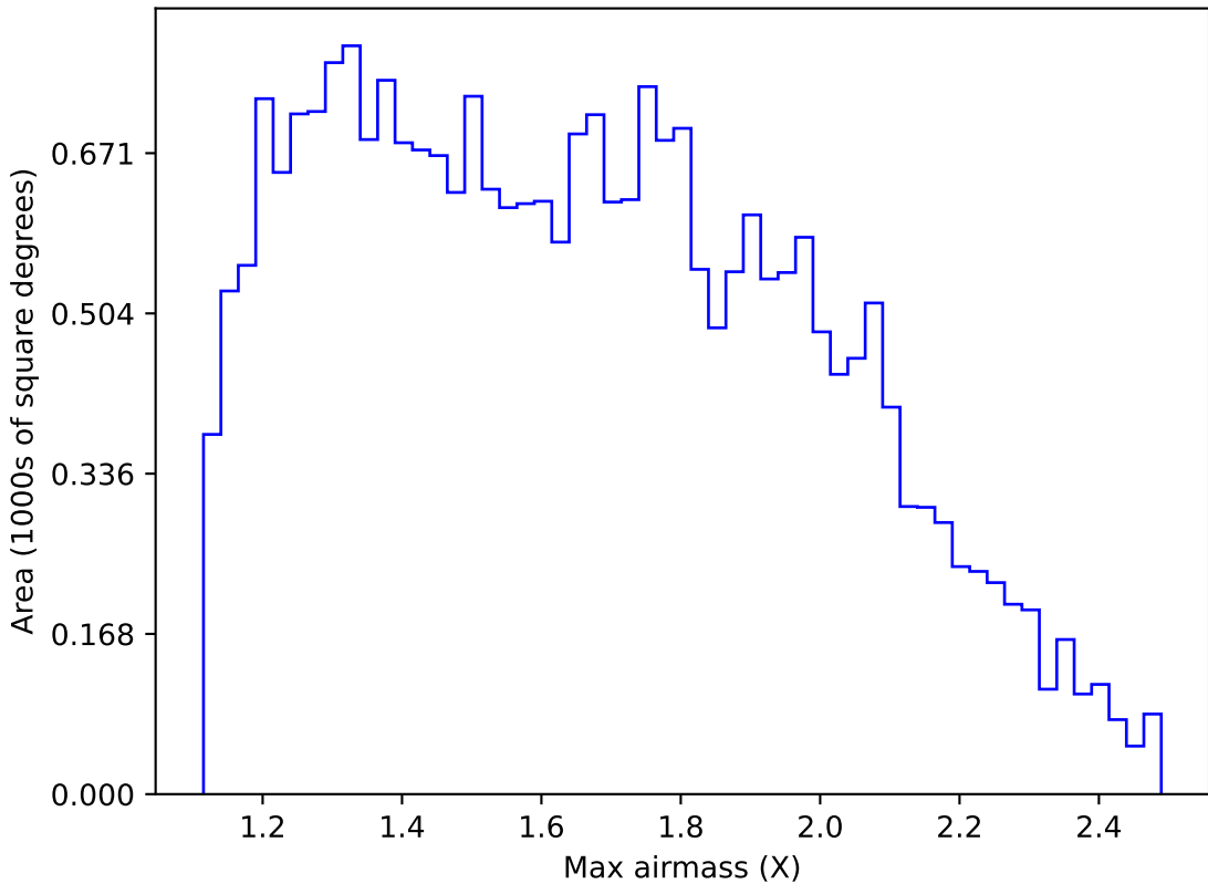
too_elab_r16_d2_ugrizy_v3.4_10yrs Yr 1 g band: Max airmass
