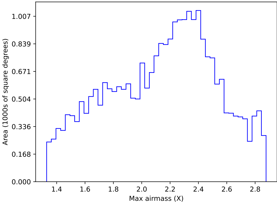
too_elab_r16_d2_ugrizy_v3.4_10yrs Yr 1 all bands: Max airmass
