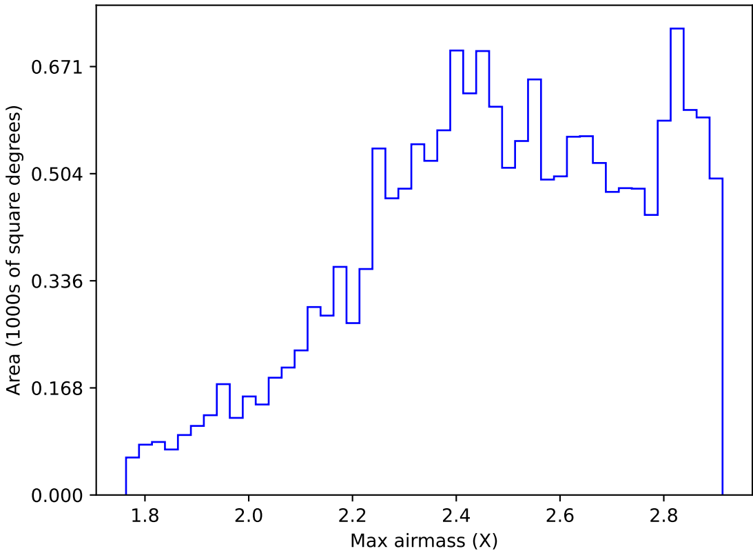
too_elab_r16_d2_ugrizy_v3.4_10yrs WFD z band: Max airmass
