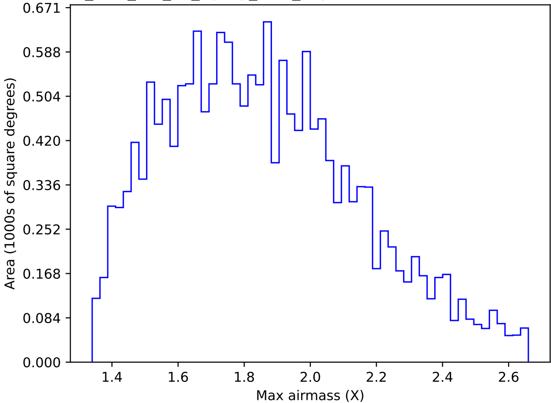
too_elab_r16_d2_ugrizy_v3.4_10yrs WFD u band: Max airmass
