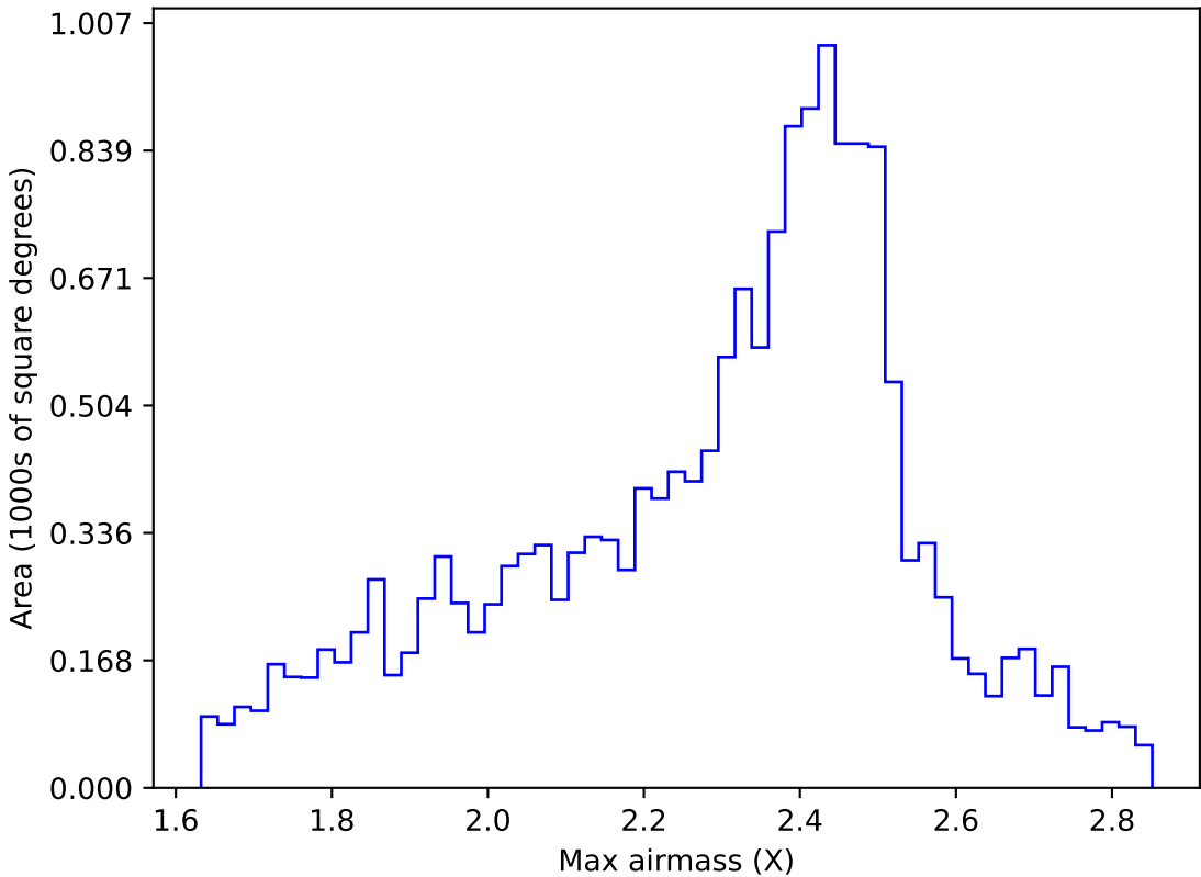
too_elab_r16_d2_ugrizy_v3.4_10yrs WFD r band: Max airmass
