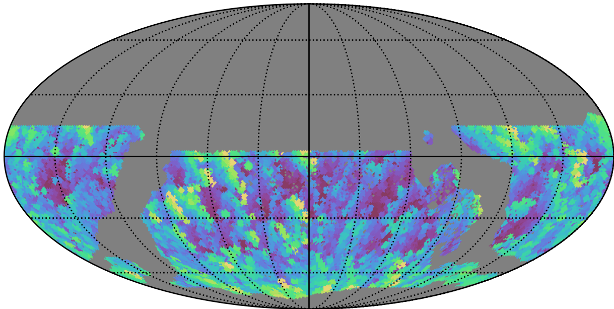
too_elab_r16_d2_ugrizy_v3.4_10yrs WFD g band: Max airmass
