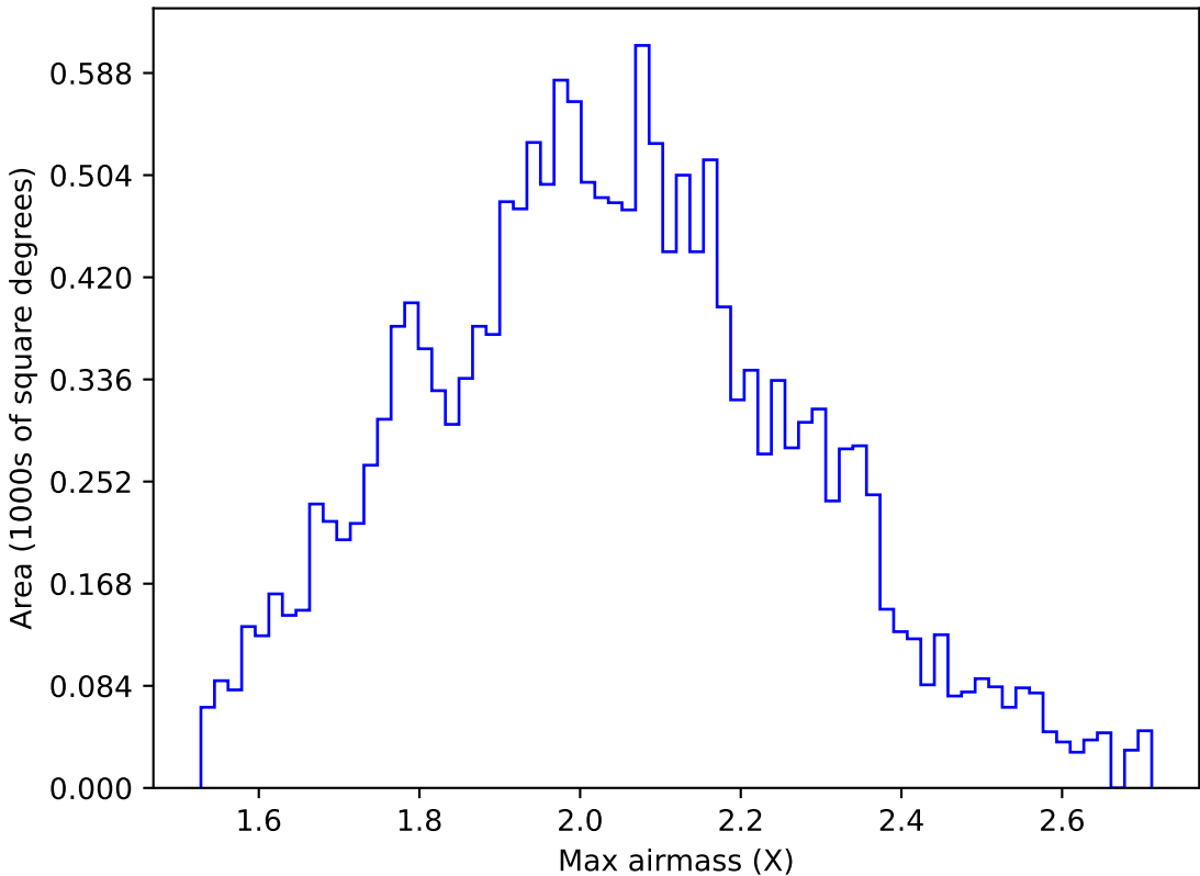
too_elab_r16_d2_ugrizy_v3.4_10yrs WFD g band: Max airmass
