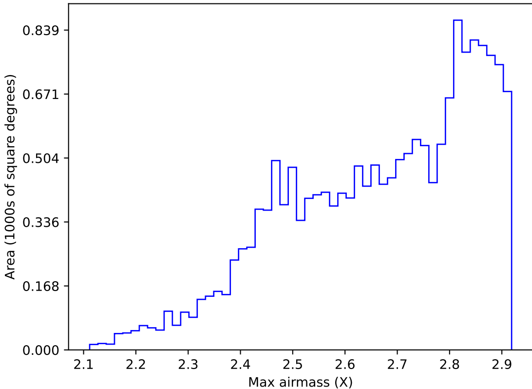
too_elab_r16_d2_ugrizy_v3.4_10yrs WFD all bands: Max airmass
