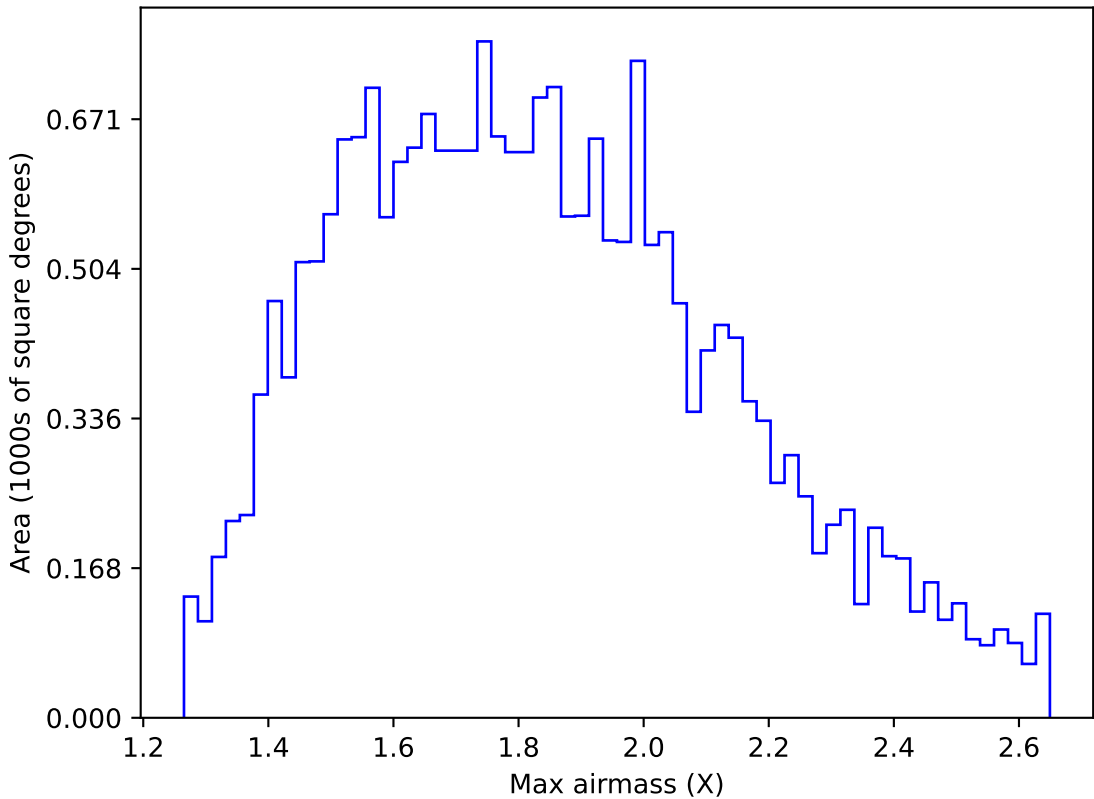
too_elab_r16_d2_ugrizy_v3.4_10yrs All sky u band: Max airmass
