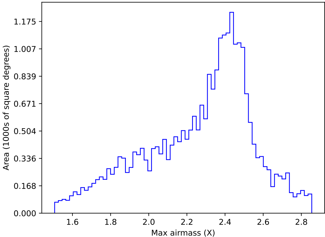
too_elab_r16_d2_ugrizy_v3.4_10yrs All sky r band: Max airmass
