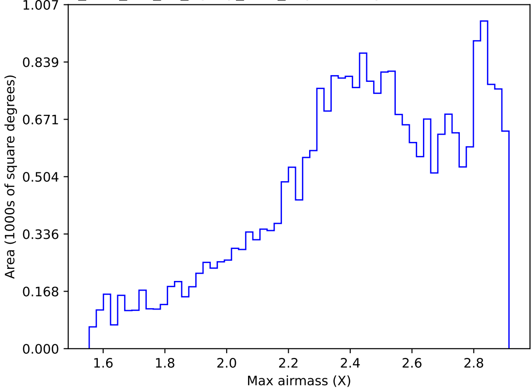
too_elab_r16_d2_ugrizy_v3.4_10yrs All sky i band: Max airmass
