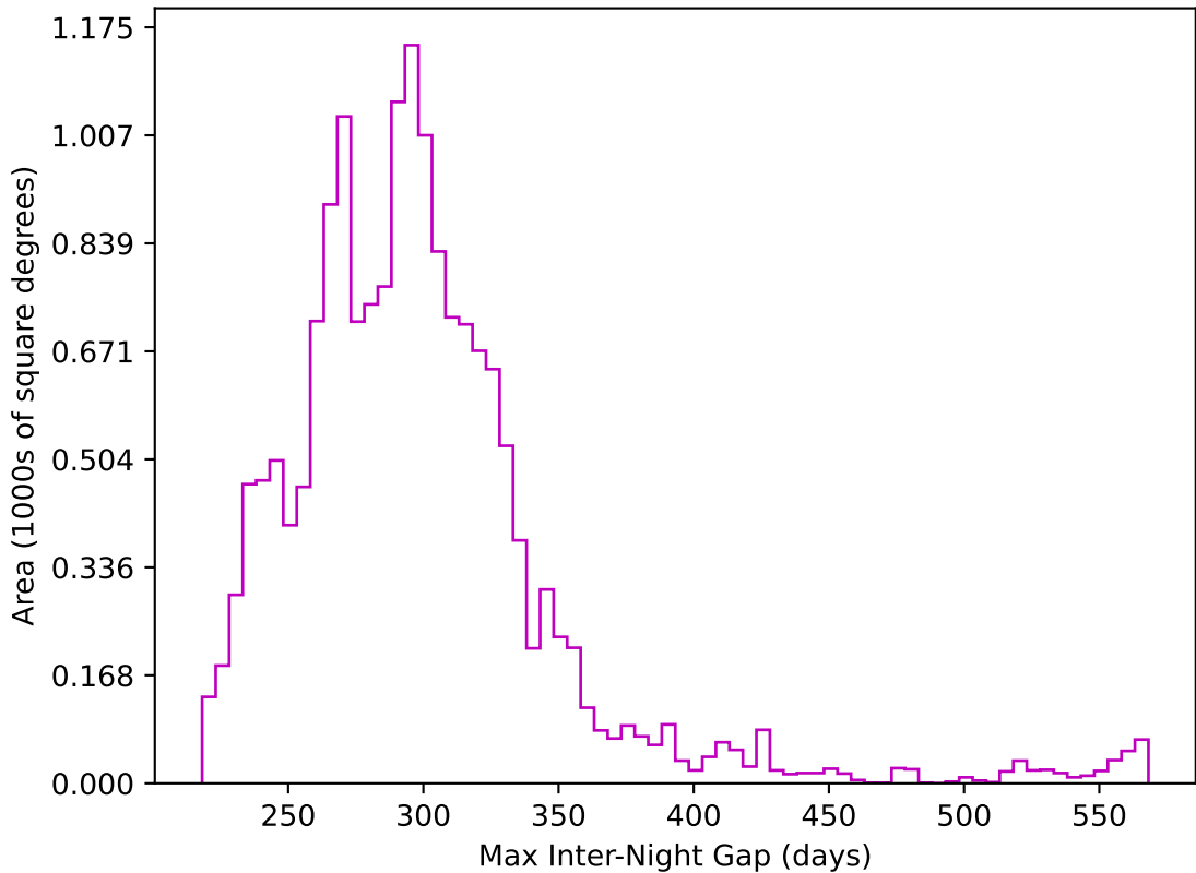
too_elab_r16_d2_ugrizy_v3.4_10yrs WFD z band: Max Inter-Night Gap
