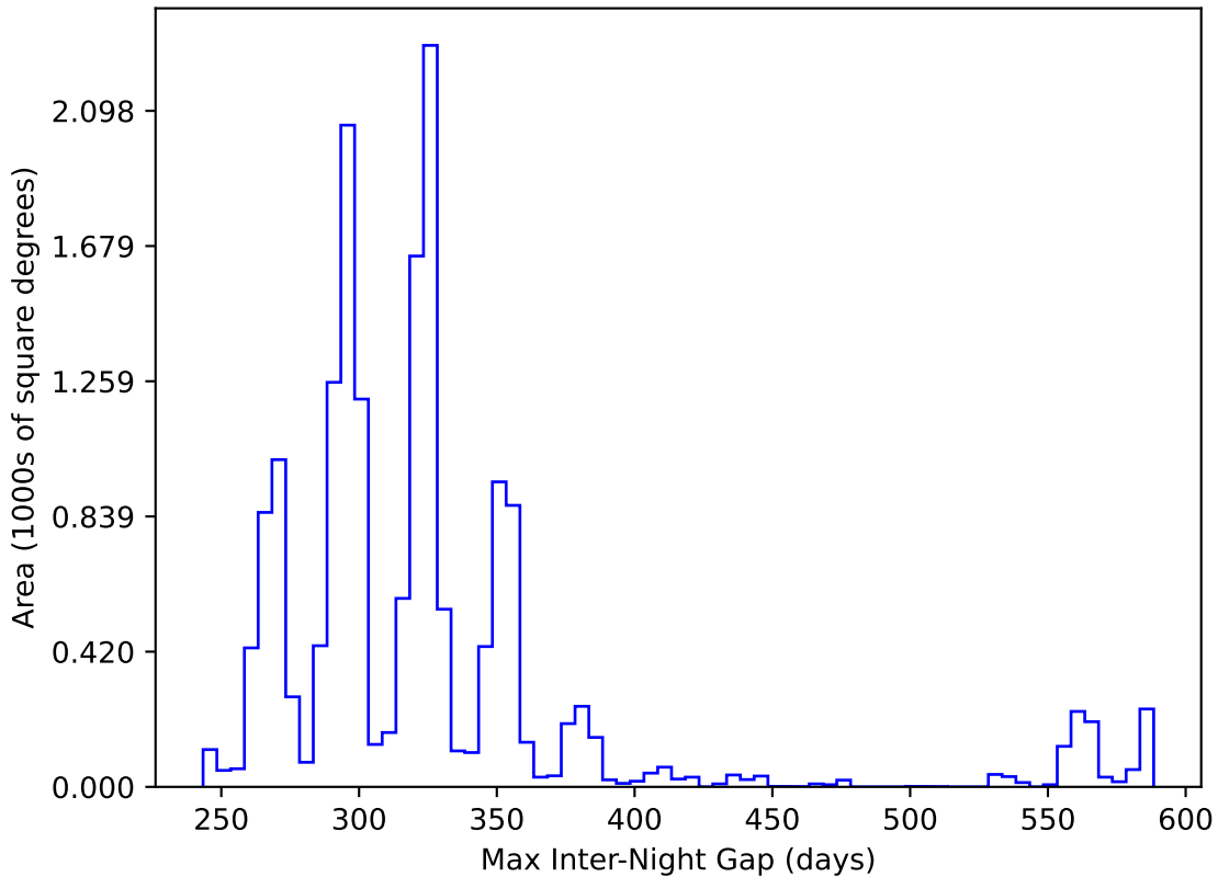
too_elab_r16_d2_ugrizy_v3.4_10yrs WFD y band: Max Inter-Night Gap
