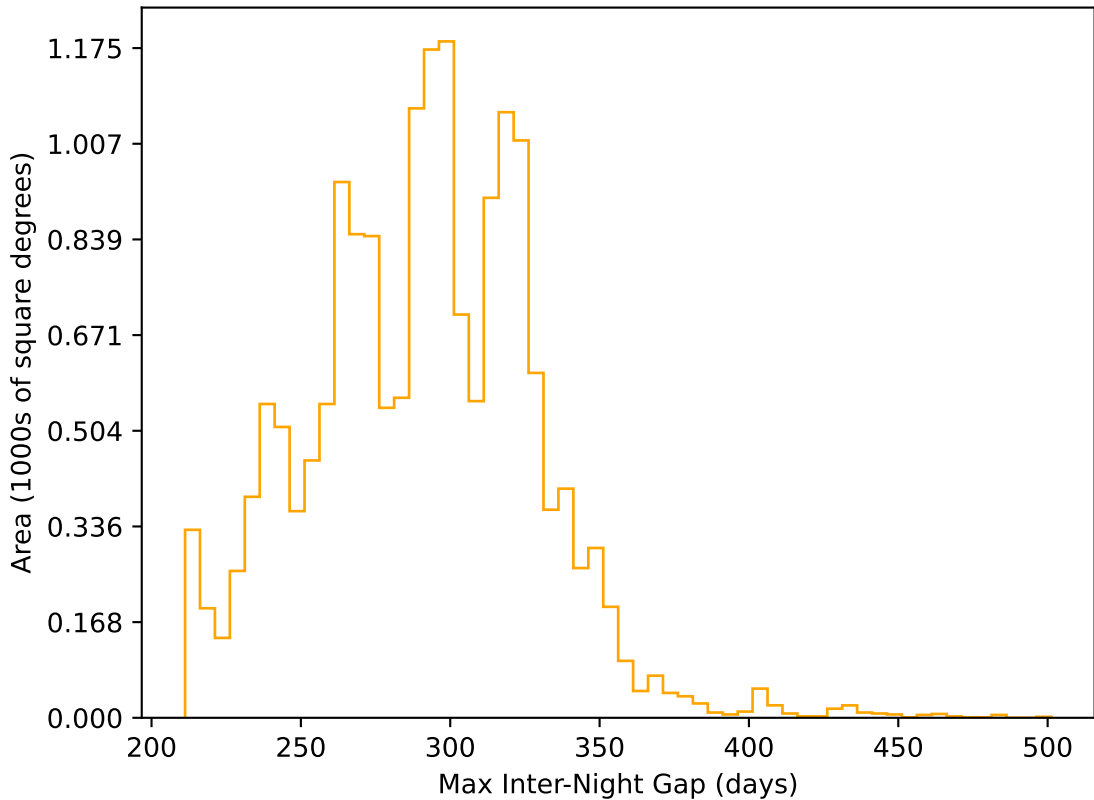
too_elab_r16_d2_ugrizy_v3.4_10yrs WFD r band: Max Inter-Night Gap
