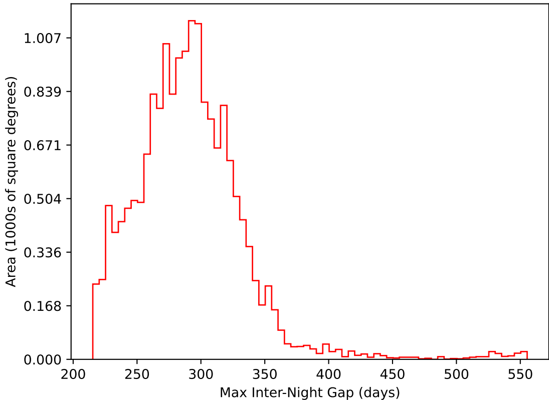
too_elab_r16_d2_ugrizy_v3.4_10yrs WFD i band: Max Inter-Night Gap
