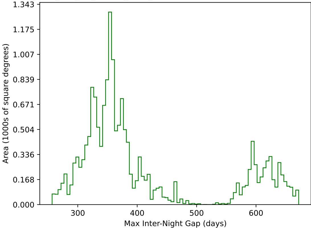
too_elab_r16_d2_ugrizy_v3.4_10yrs WFD g band: Max Inter-Night Gap
