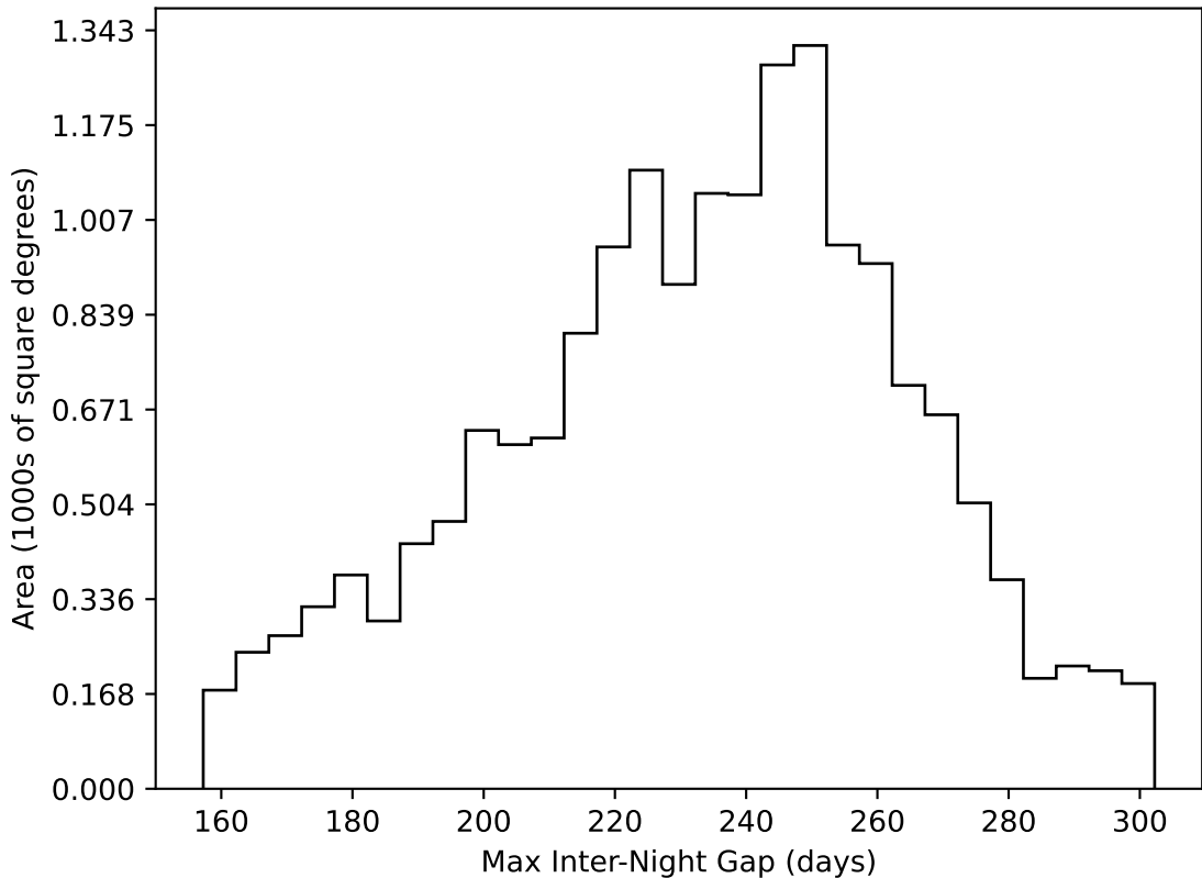
too_elab_r16_d2_ugrizy_v3.4_10yrs WFD all bands: Max Inter-Night Gap
