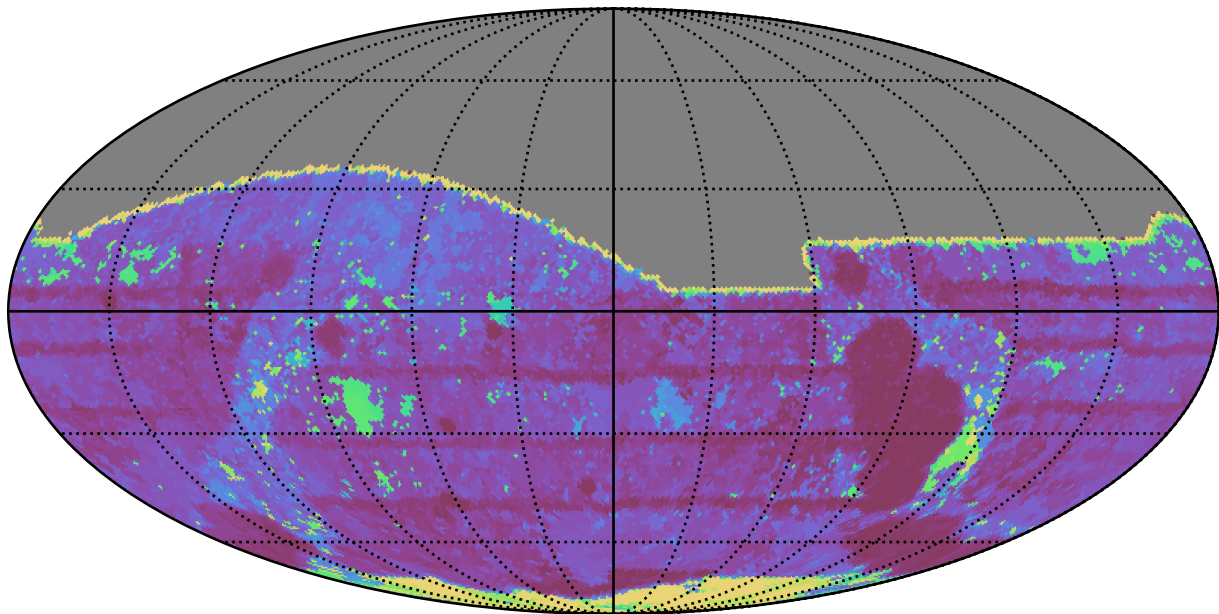
too_elab_r16_d2_ugrizy_v3.4_10yrs All sky r band: Max Inter-Night Gap
