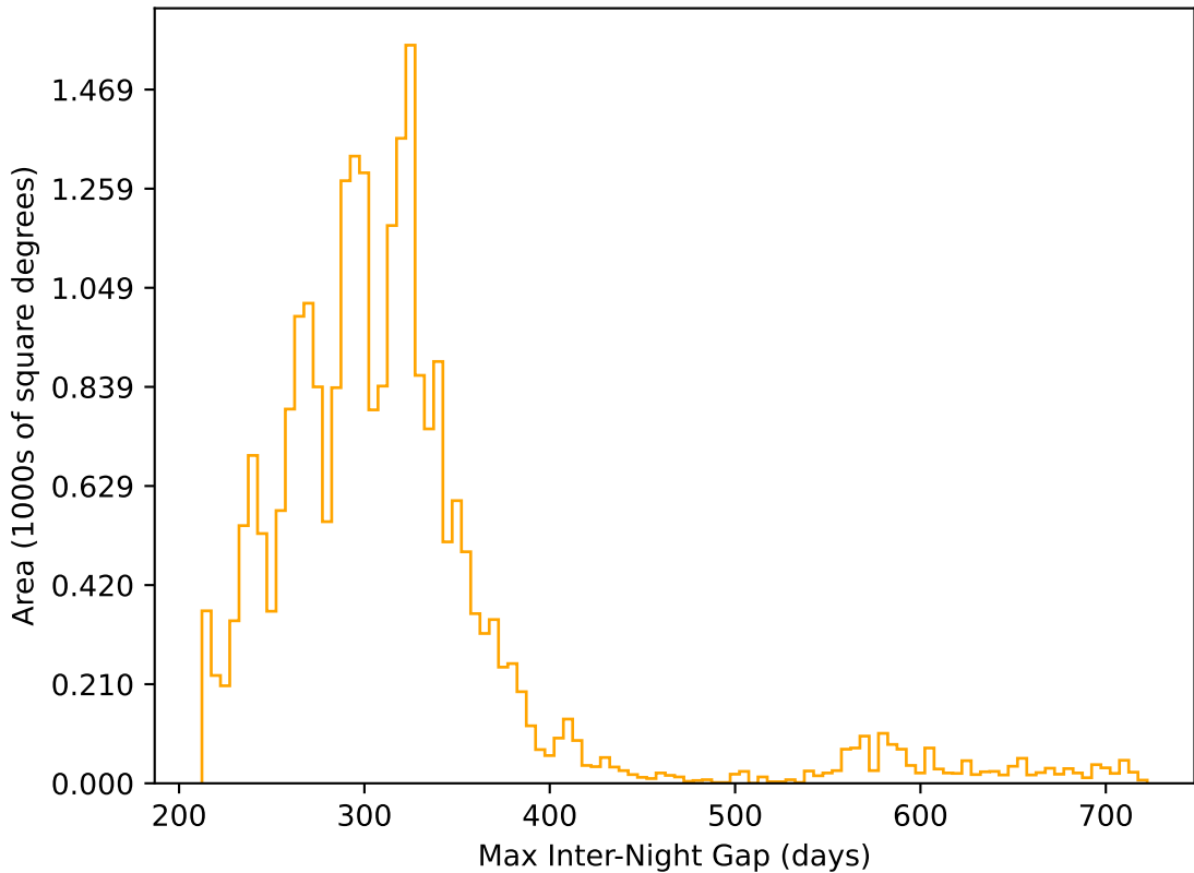
too_elab_r16_d2_ugrizy_v3.4_10yrs All sky r band: Max Inter-Night Gap
