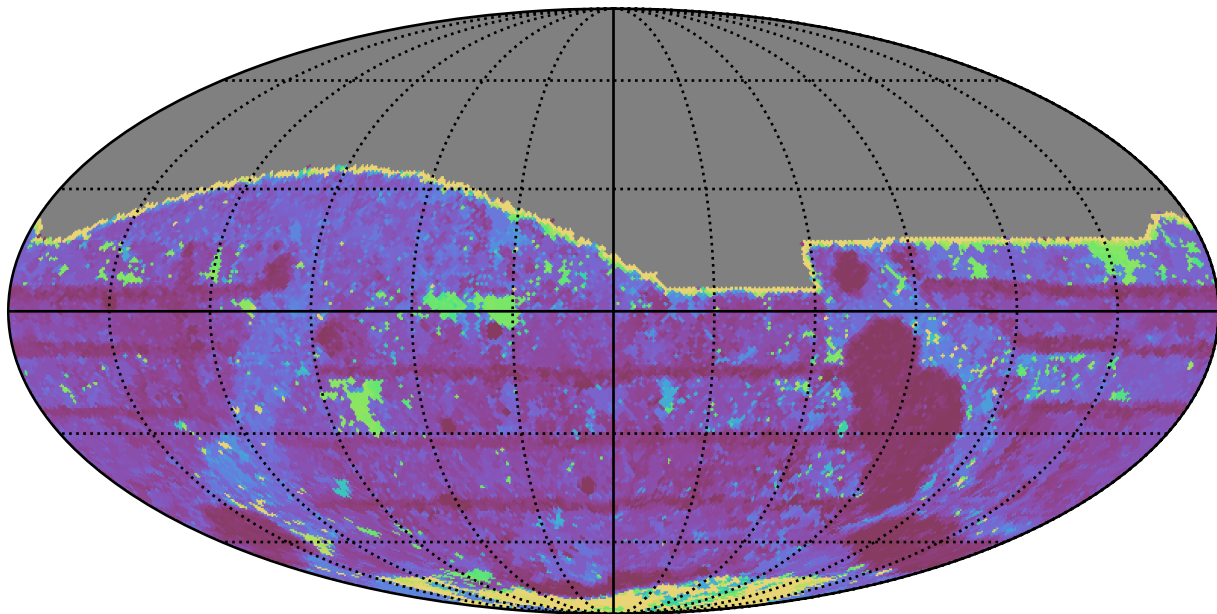
too_elab_r16_d2_ugrizy_v3.4_10yrs All sky i band: Max Inter-Night Gap
