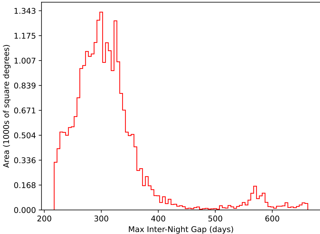
too_elab_r16_d2_ugrizy_v3.4_10yrs All sky i band: Max Inter-Night Gap
