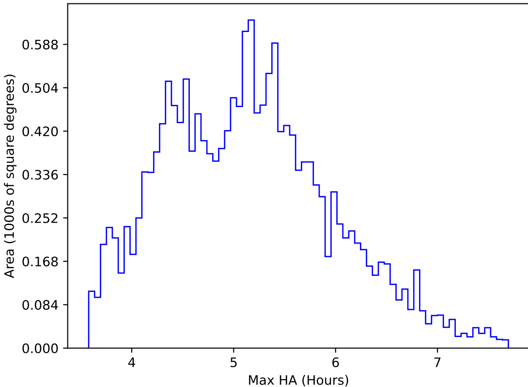
too_elab_r16_d2_ugrizy_v3.4_10yrs WFD all bands: Max HA
