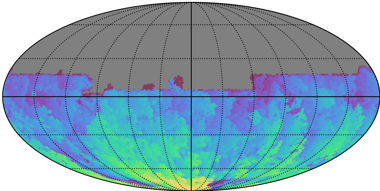
too_elab_r16_d2_ugrizy_v3.4_10yrs All sky u band: Max HA
