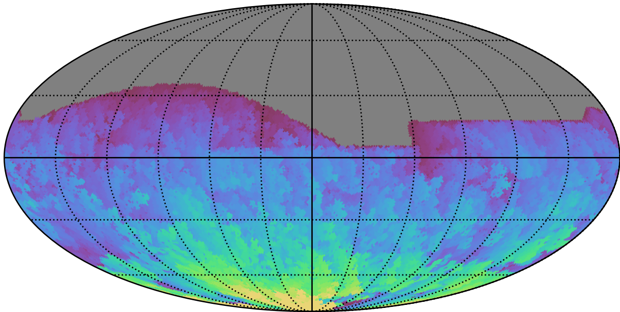
too_elab_r16_d2_ugrizy_v3.4_10yrs All sky r band: Max HA
