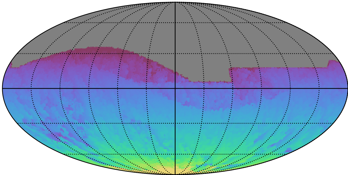
too_elab_r16_d2_ugrizy_v3.4_10yrs All sky all bands: Max HA
