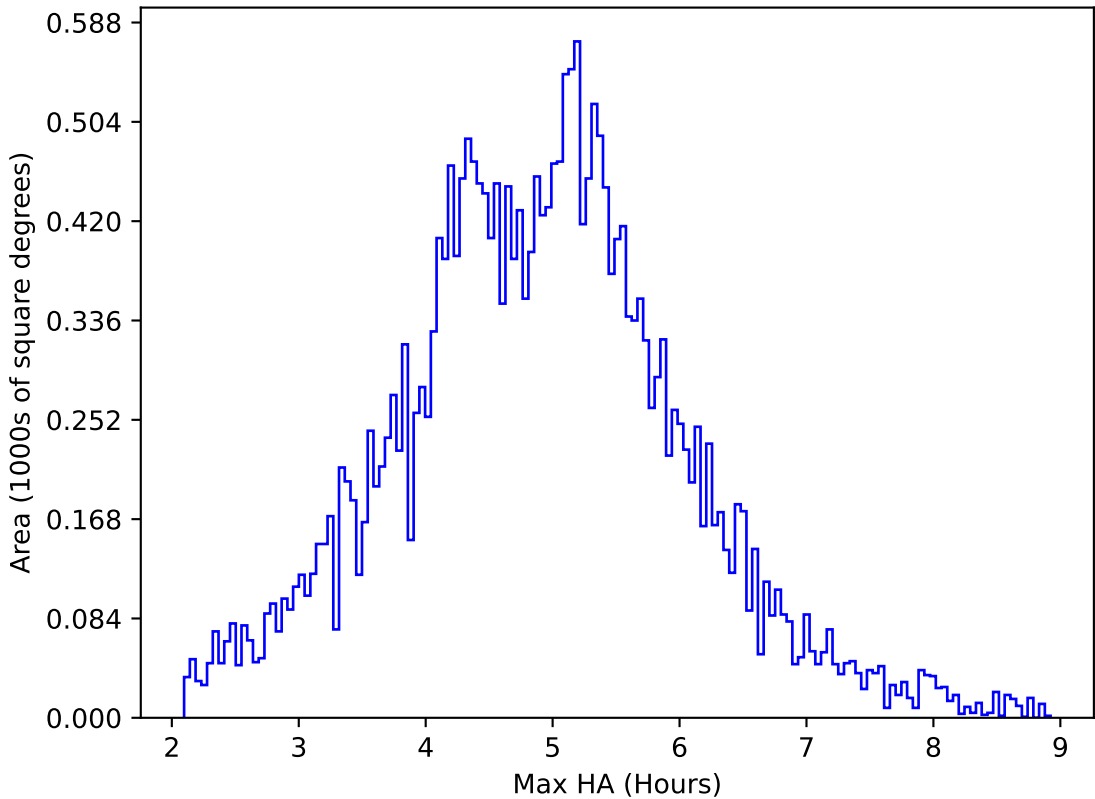
too_elab_r16_d2_ugrizy_v3.4_10yrs All sky all bands: Max HA
