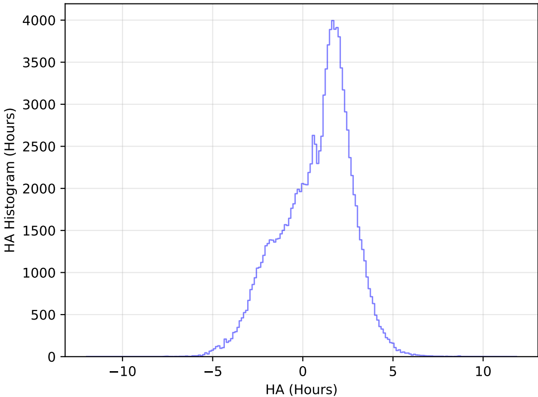
too_elab_r16_d2_ugrizy_v3.4_10yrs WFD u band: HA Histogram
