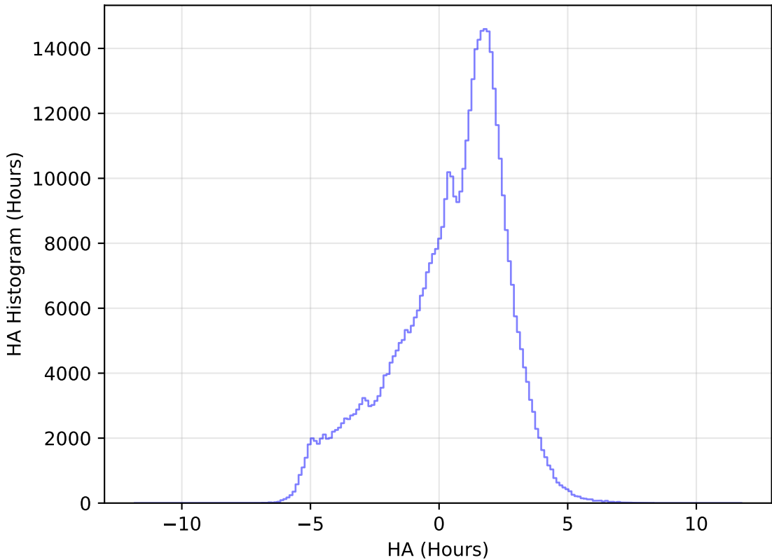
too_elab_r16_d2_ugrizy_v3.4_10yrs WFD r band: HA Histogram
