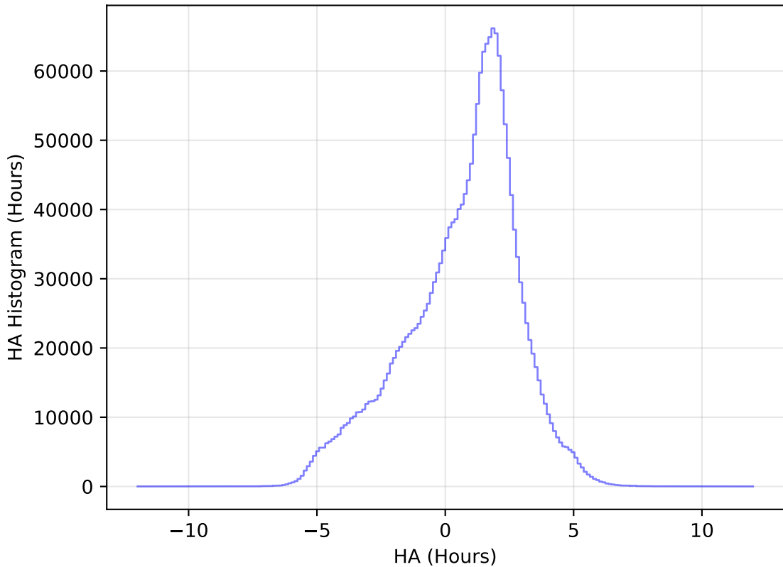
too_elab_r16_d2_ugrizy_v3.4_10yrs WFD all bands: HA Histogram
