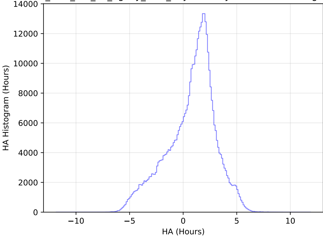
too_elab_r16_d2_ugrizy_v3.4_10yrs All sky z band: HA Histogram
