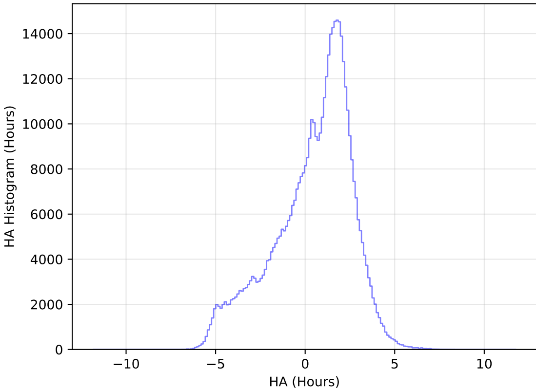
too_elab_r16_d2_ugrizy_v3.4_10yrs All sky r band: HA Histogram
