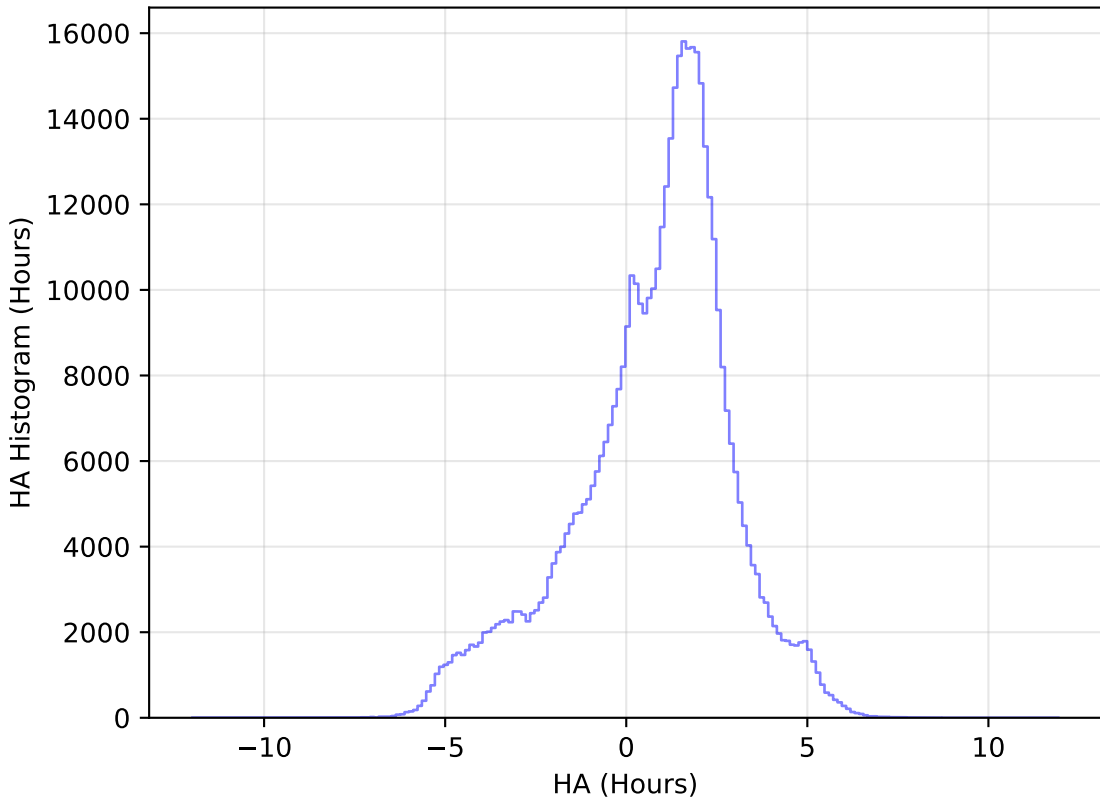
too_elab_r16_d2_ugrizy_v3.4_10yrs All sky i band: HA Histogram
