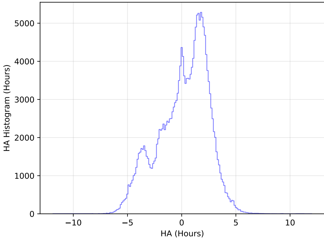
too_elab_r16_d2_ugrizy_v3.4_10yrs All sky g band: HA Histogram
