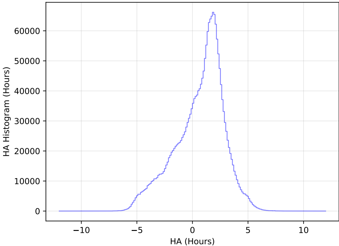
too_elab_r16_d2_ugrizy_v3.4_10yrs All sky all bands: HA Histogram
