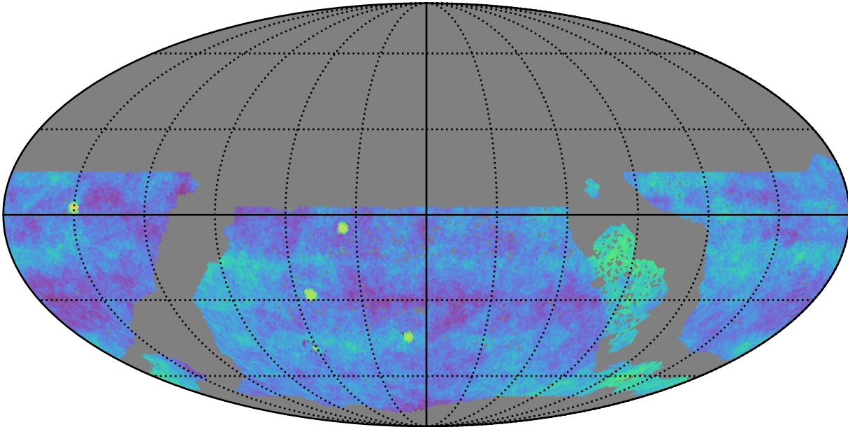
too_elab_r16_d2_ugrizy_v3.4_10yrs gri WFD: Fraction of visits in pairs (20-90 min)
