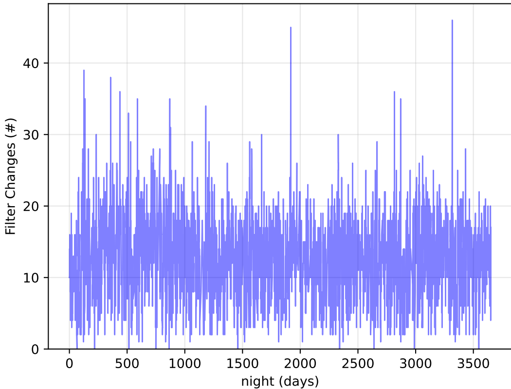
too_elab_r16_d2_ugrizy_v3.4_10yrs Per Night: Filter Changes
