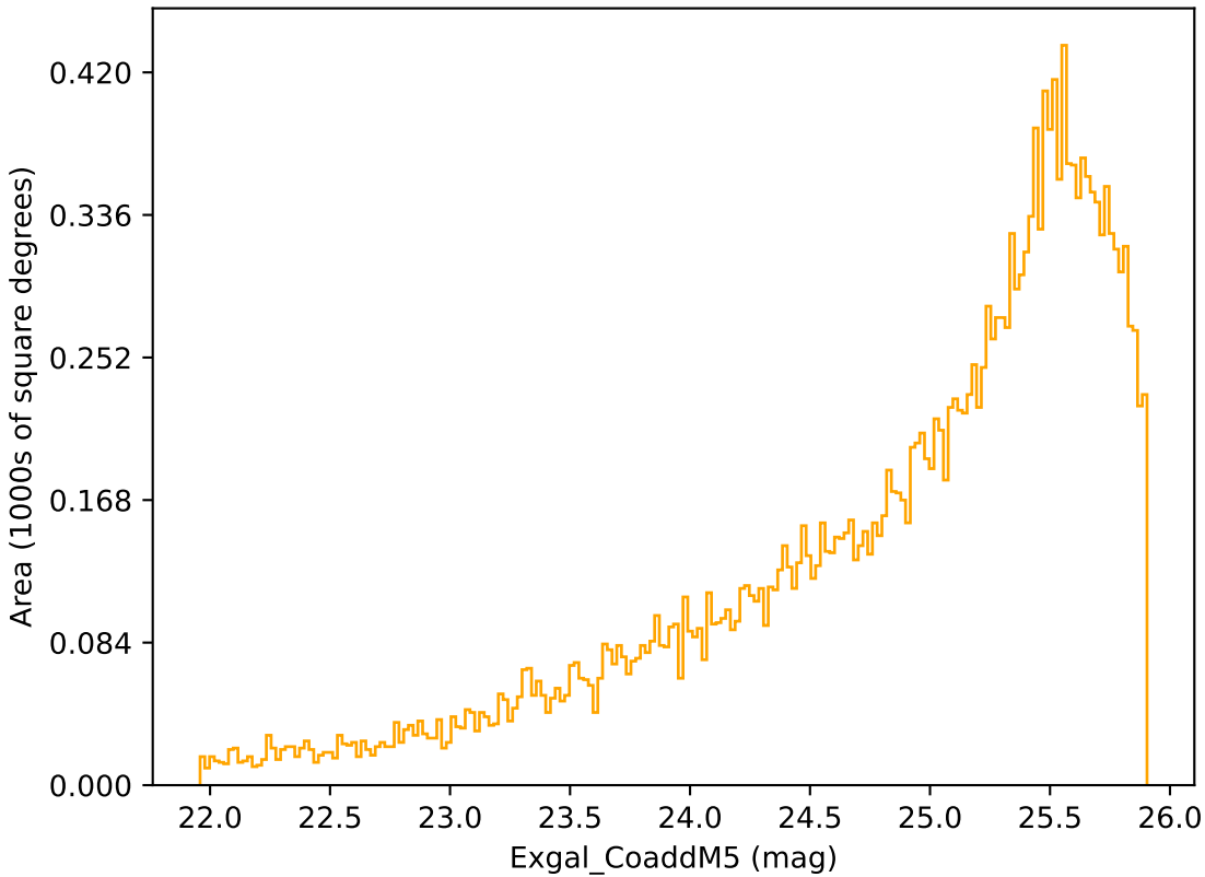
too_elab_r16_d2_ugrizy_v3.4_10yrs Yr 3-4 r band: Exgal_CoaddM5
