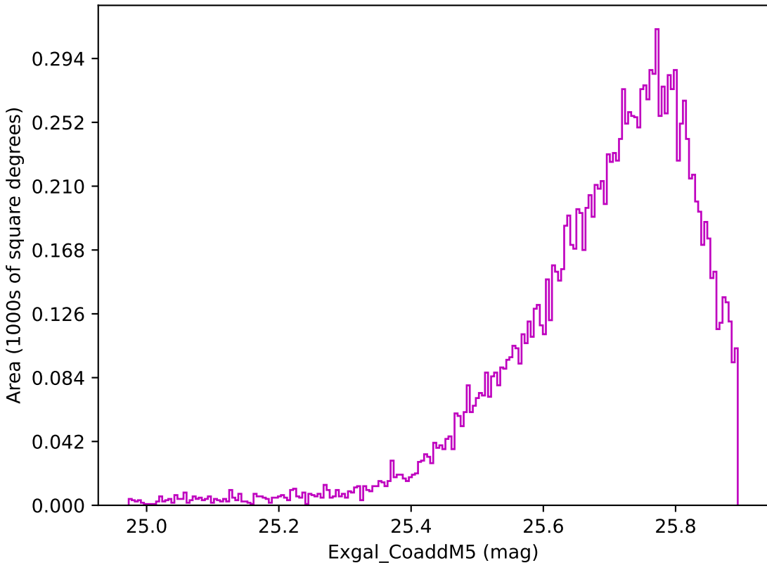
too_elab_r16_d2_ugrizy_v3.4_10yrs WFD z band: Exgal_CoaddM5
