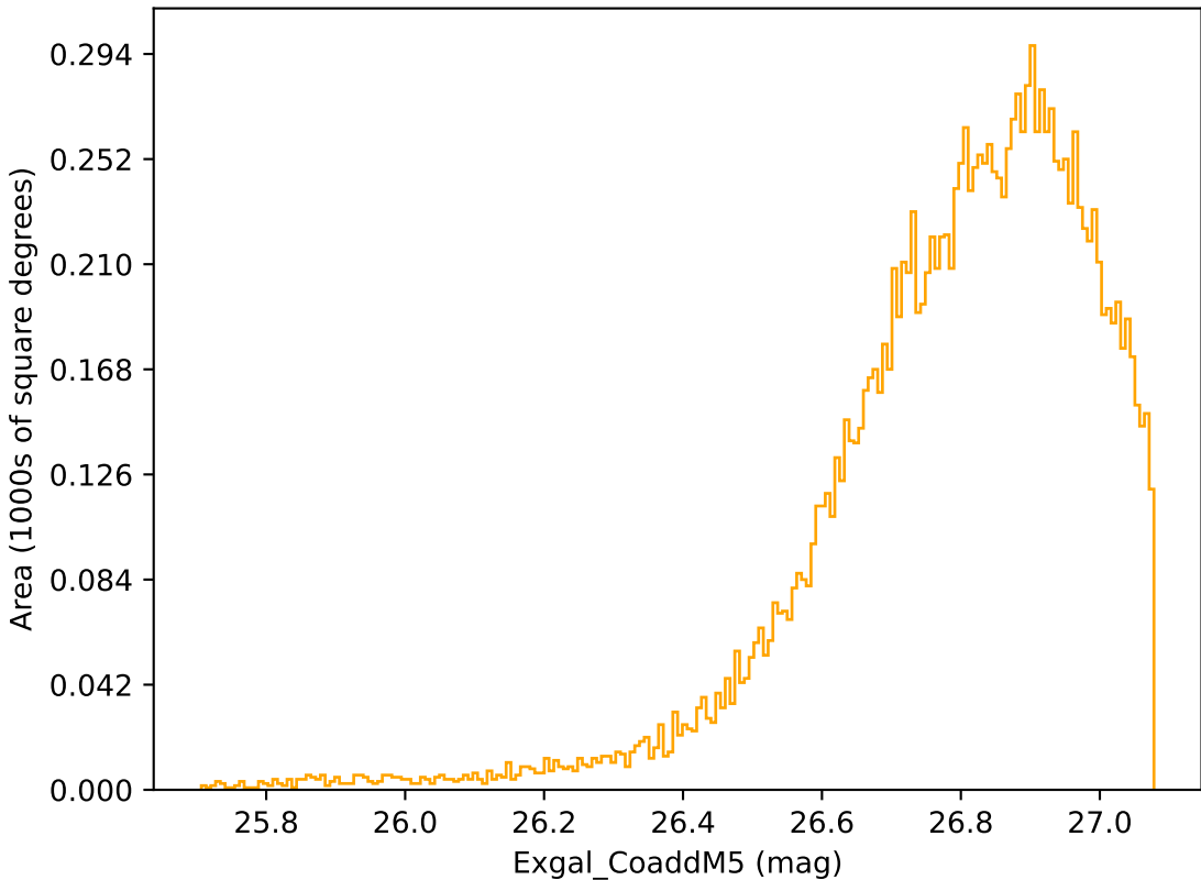
too_elab_r16_d2_ugrizy_v3.4_10yrs WFD r band: Exgal_CoaddM5
